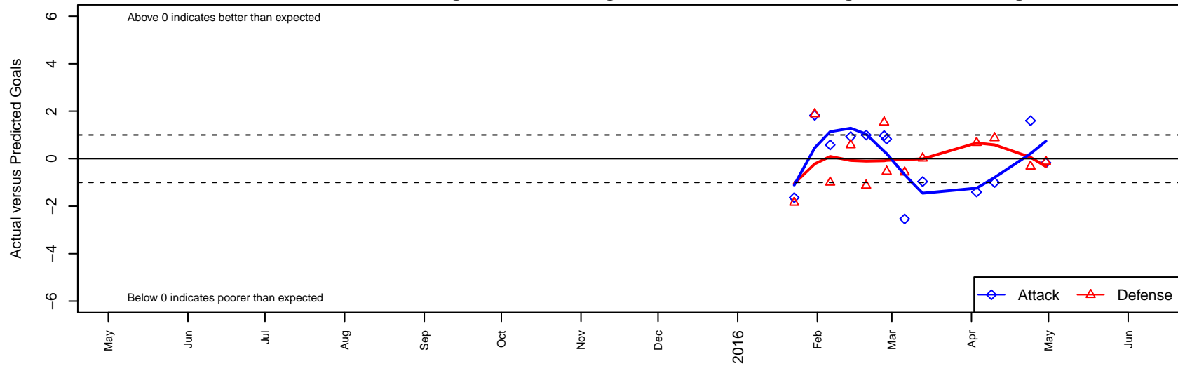
NICH SC Impact B98 Dots are actual minus expected GF (blue circles) and GA (red triangles). Blue line is smoothed change in attack strength. Red is smoothed change in defense strength.
